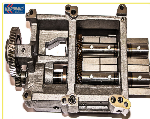
Balancer Unit
