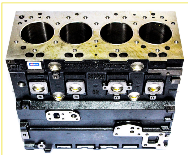
Cylinder Block
