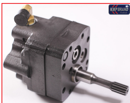
Fuel Pump Gear 3/4
