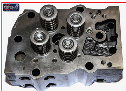
Cylinder Head (Loaded)
