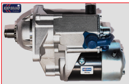
Starter Motor 24V 4.5Kw 10T
