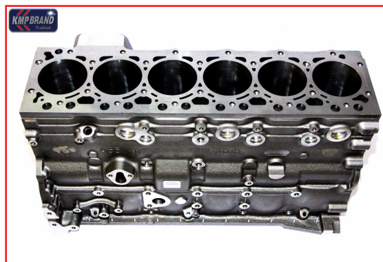
Cylinder Block
