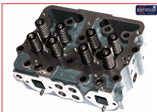
Cylinder Head (Loaded)
