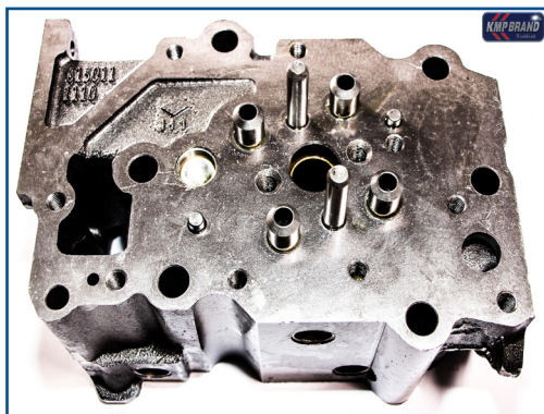
Cylinder Head (Bare)
