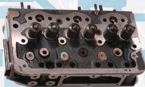
CYLINDER HEAD
